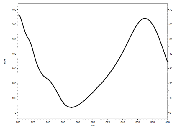
UV of Xanthohumol ICS-X1 at 370 nm and RT 4.0 min.
