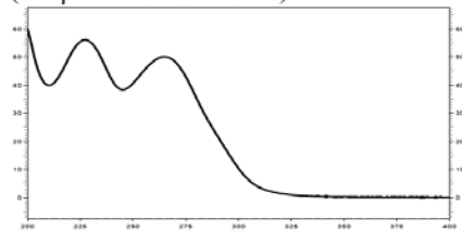
2nd Rho Peak at 3.67 min. (cis-p-isocohumulone 2)
